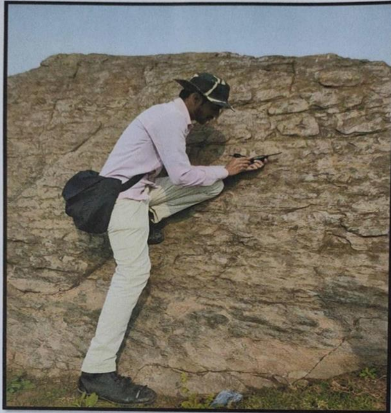
Measuring the trends of strata by M.Sc. Geoinformatics students for Ground truthing of data
