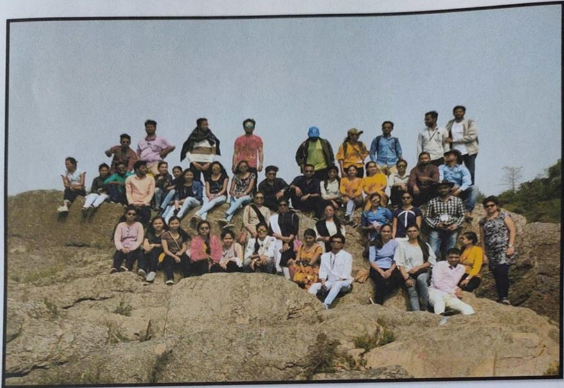
Geological Fieldwork in Lameta Ghat (M.P) area.
