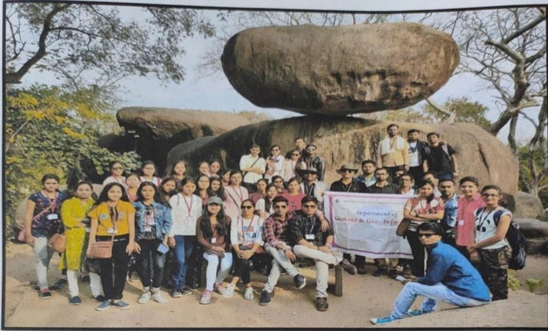
Geological Fieldwork @ Balance Rock (Granite Plutons) Madan Mahal area, Jabalpur (M.P)
