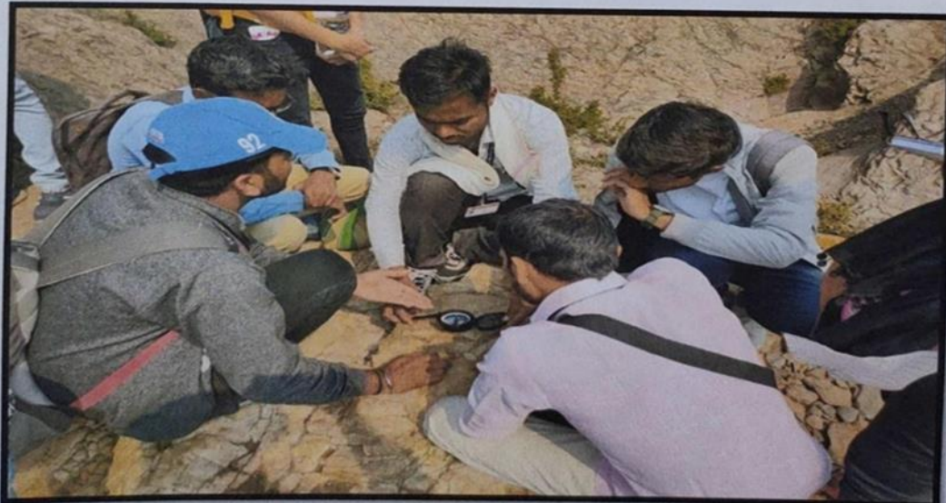
Measuring the strike and dip of strata by B.Sc. Geology students with the help of Brunton compass
