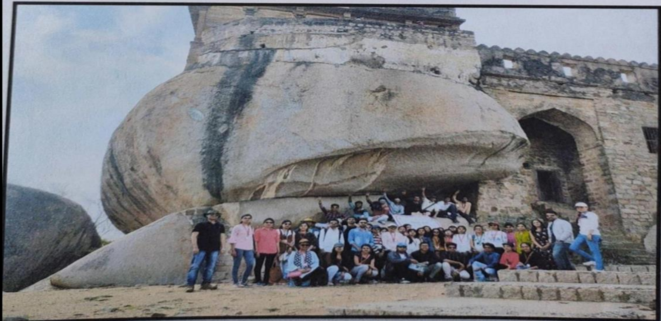
Geological Fieldwork @ Madan Mahal area, Jabalpur (M.P)
